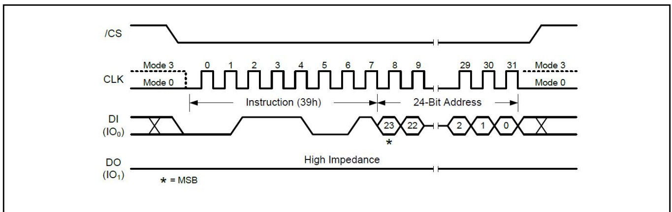
Figure 37. Individual Block Unlock Instruction for SPI Mode
